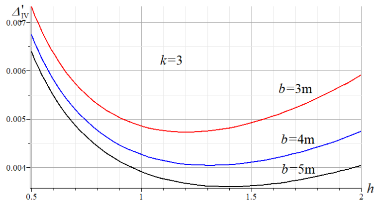
Figure 9. Dependence of the deflection of the truss on the action of the wind load on the height.
